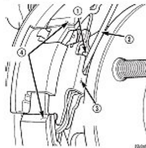
Fig. 68 Parking Brake
