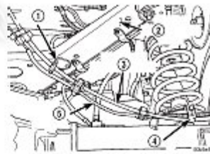
Fig. 67 Left Rear Parking Brake Cable
